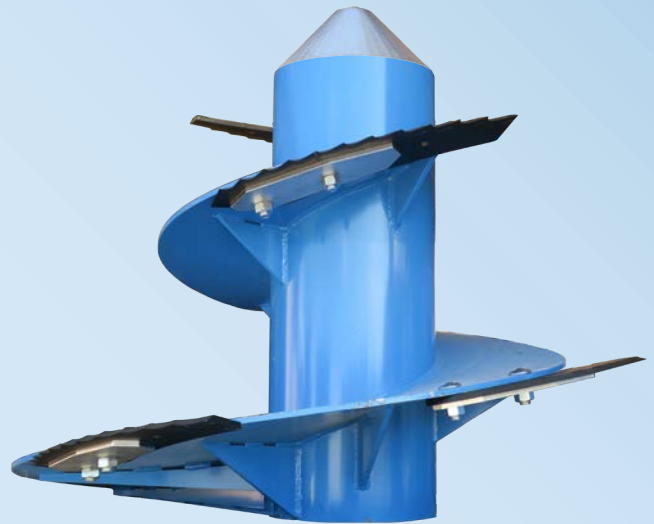
Augers are built using 3/8" thick stainless steel flight with braces along the bottom side. In addition, at the top knife (a high stress area) the flight is double thickness, for a total thickness of 3/4".
